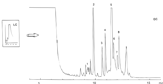
Figure 3. Liquid chromatogram of sunflower oil and gas chromatogram obtained after transfer of the indicated fraction (3416 \mu\text{L} of methanol–water eluent, 78:22) under the experimental conditions giving the best response in the optimization procedure (vertex 6 in Table 2). Identification peak number as in Figure 1. (HPLC flow rate, 2000 \mu\text{L}/\text{min} ).
